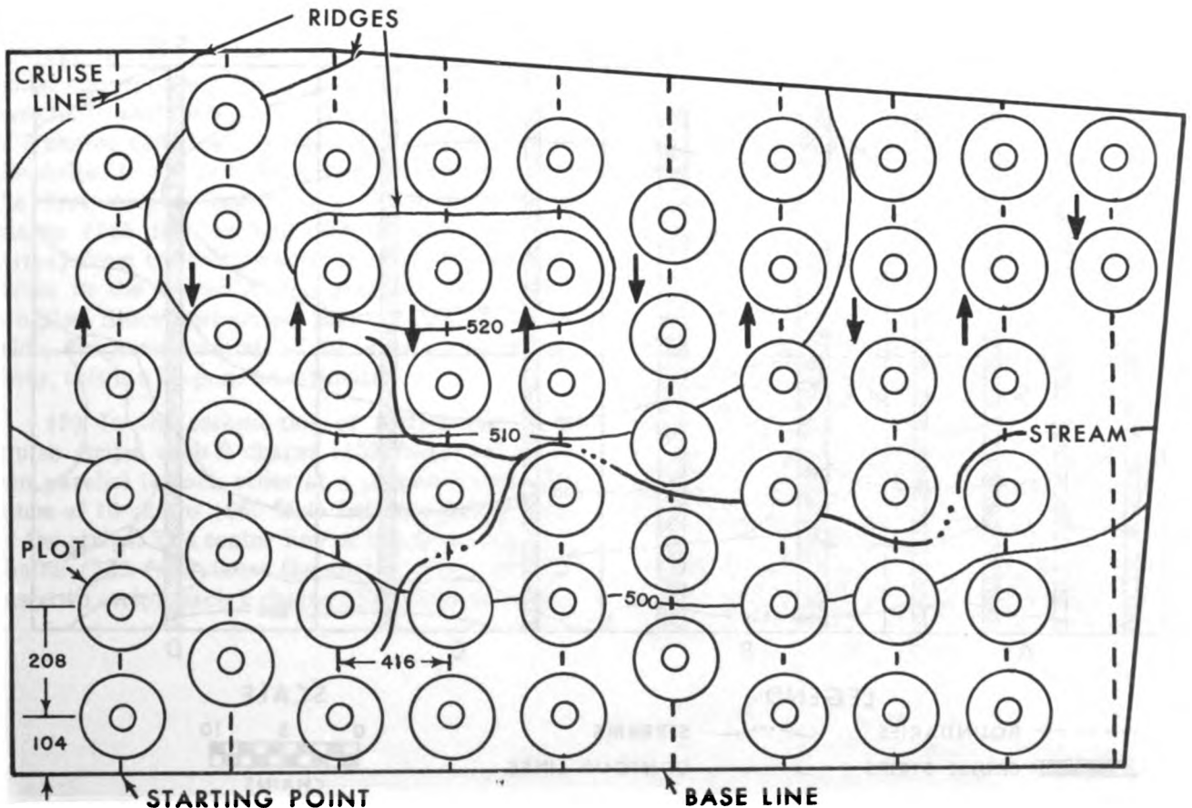
Figure 2-10. Plot method of estimating timber.
